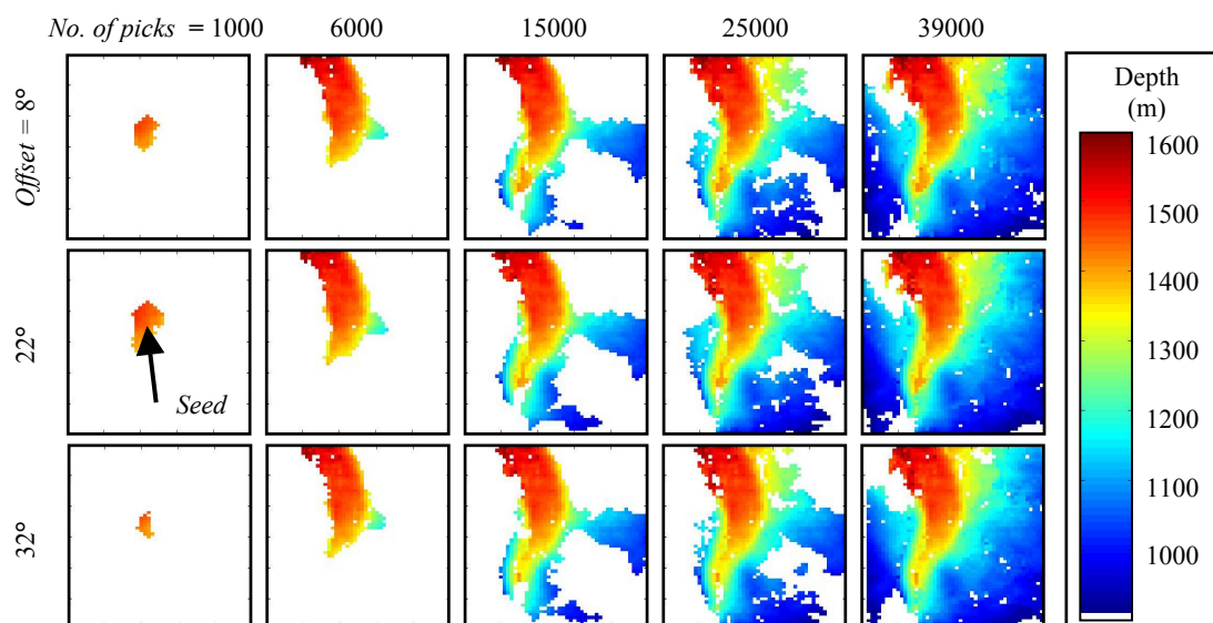
Figure 2. Evolution of the picked reflection event in prestack hyperspace. Areas that have not been picked are shown in white. The picked surface grows in 4-D based on a quantitative assessment of previously made picks.
