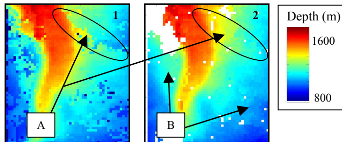
Figure 4. Comparison between hyperspace propagation using flow features and correlation autopicking results for two constant offset lines. The correlation autopicker has produced loop skipping. The 4-D constraints enforced by the propagator avoid this problem and track the event despite the varying signal-to-noise ratio.
