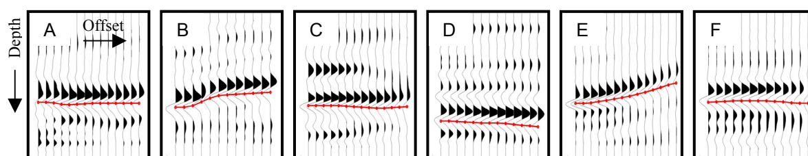
Figure 1. A range of residual moveout trends have been accurately picked. This includes non-hyperbolic trends (B). Autopicked events are shown in red.
