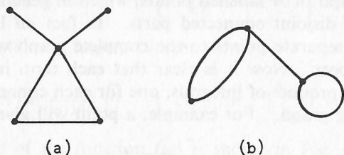
Figure 5. (a) simple graphs; (b) not simple graphs
